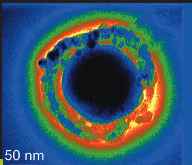
Energy-filtered TEM image of a single Au/TiO 2 nanocap.
